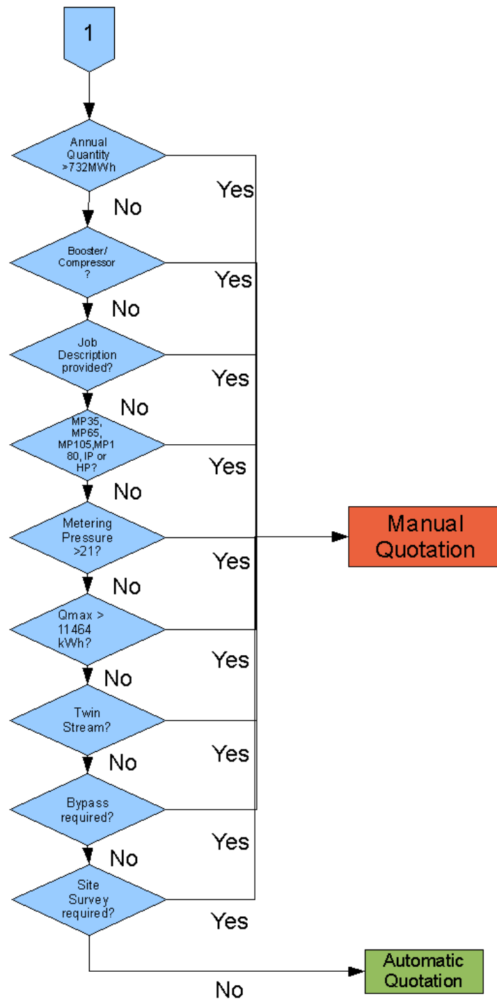
Illustration 9: Automatic or Manual Quotation Flow Chart 2
