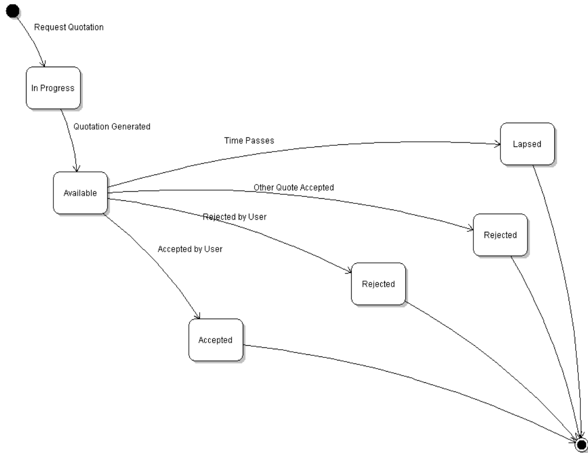
Illustration 10: Quotation State Diagram
